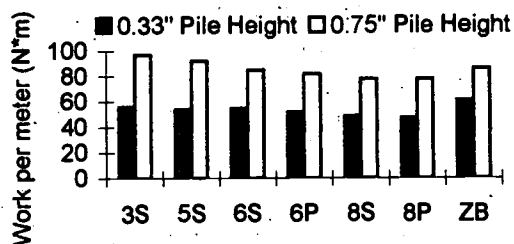
Figure 2. Work required on two carpet types
