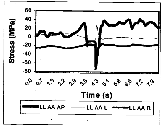
Figure 1. Plot of stress at above-ankle gages vs. time during ambulation task.
