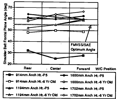
Figure 4: Shoulder Belt Frontal Plane Torso Angle for P5 Female and 6 Year Old Occupants compared to FMVSS/SAE Optimum Angle
