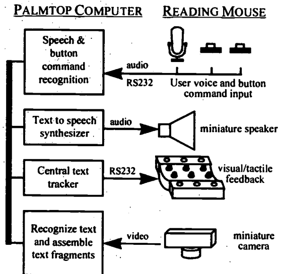
Fig. 1 - IRA system components
