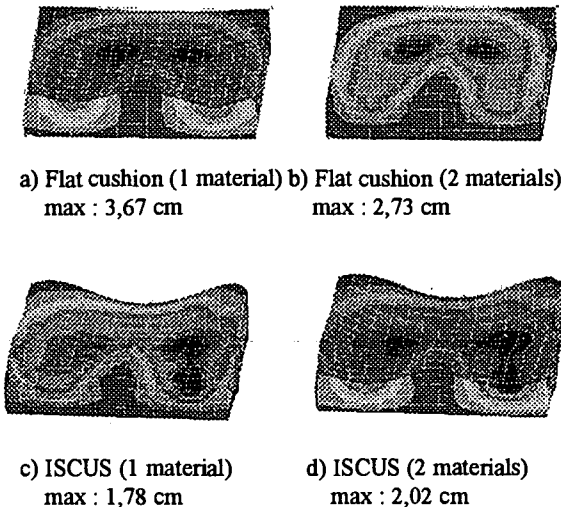
Figure 3: Vertical displacements obtained from simulations of a real subject pressure applied on different cushion models
