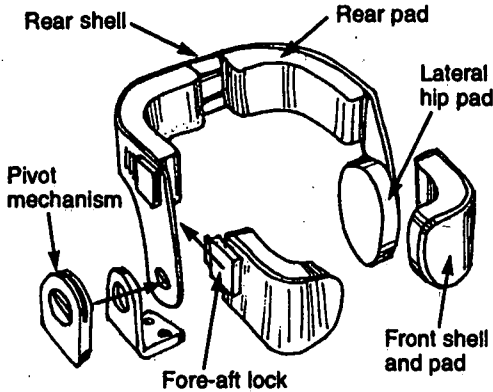
Figure 1. The Hip Grip
