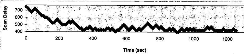
Figure 5. Scan delay for subject MM for a trial with automatic adaptation active.
