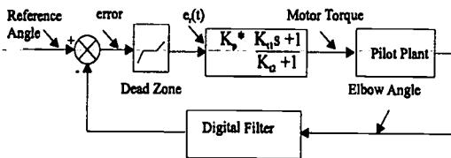
Figure 2: Lead-lag controller
