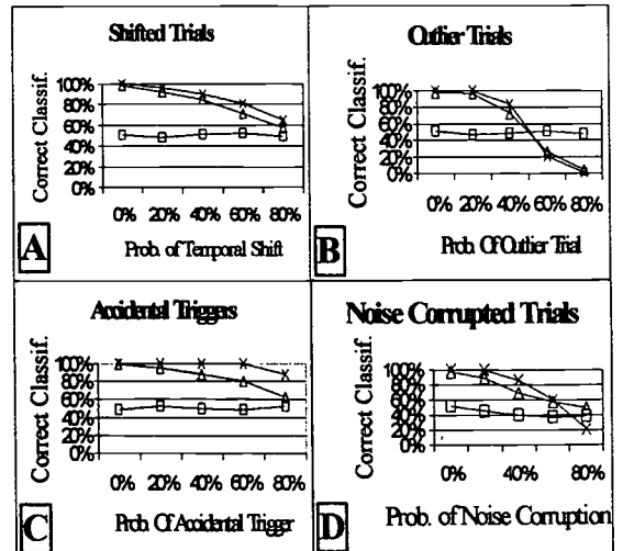
Figure 2 – Results of sorting method applied to simulated data. The lines are coded as follows: true SNR 0.1 "□", true SNR 1.0 "△", and true SNR 10 "×".
