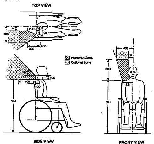
Figure 1: SAE J2249 Preferred and optional zones for upper vehicle anchor point of shoulder restraint [1].
