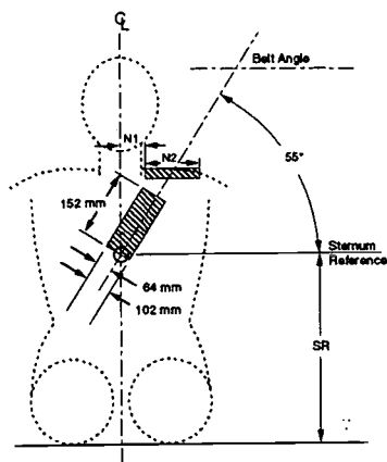
Figure 2: Preferred zones for location of shoulder belt on occupant's torso [1,2].
