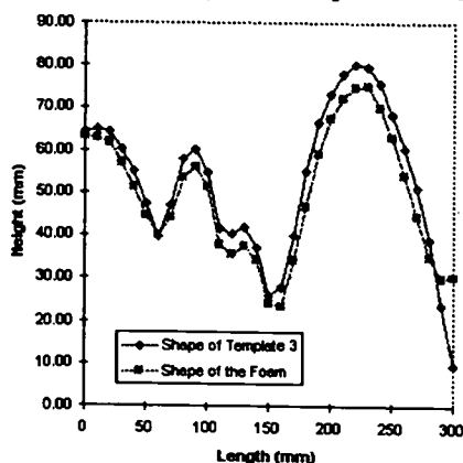
Figure 2. Shape comparison between curved templates and the associated foam copies
