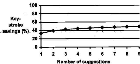
Figure 1. Keystroke savings as a function of the number of suggestions.
