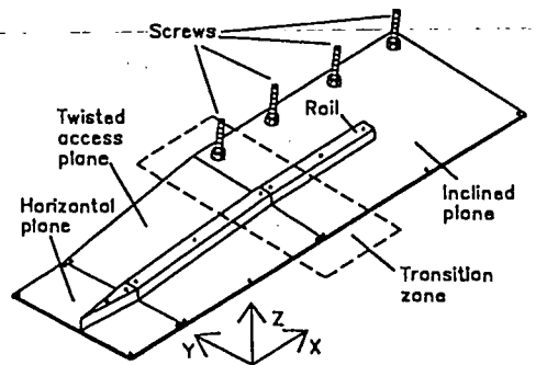
Figure 1. Schematic representation of the experimental pathway designed to allow lateral tilt of the wheelchair.
