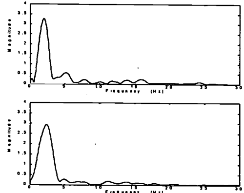
Figure 3. The gain of the transfer function of the whole body acceleration system for bump #3 in trial 3: top -- with cushion; bottom -- without cushion)
