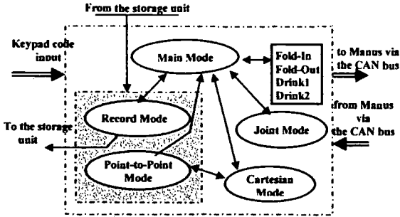
Figure 2: A new mode control organization
