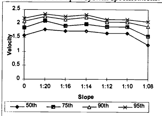
Figure 3. Distribution of velocity as a function of ramp slope.
