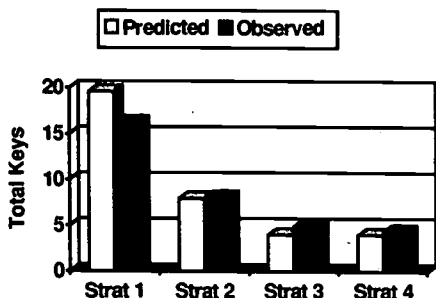
Figure 1: Avg. total on-screen keyboard keys required to accomplish each selection task
