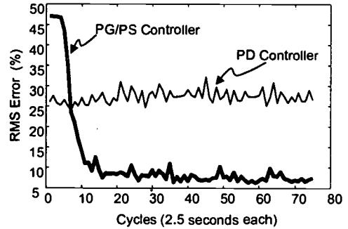
Figure 4: Example of RMS errors across cycles for both controllers seen in Figure 3. (The trials with the lowest mean RMS error over the last 10 cycles define best performance.)
