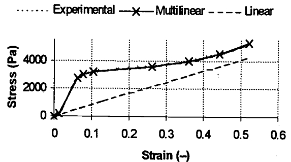
Figure 1: Modeled and experimental mechanical properties of foam
