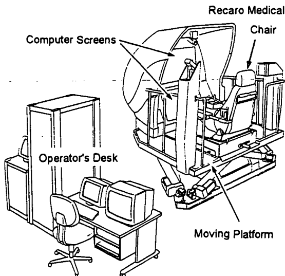
Fig. 1 The simulator of powered wheelchair.
