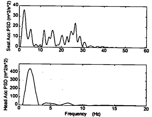
Figure 2. PSD of the acceleration during the bump #3 in the trial 3 with cushion.
