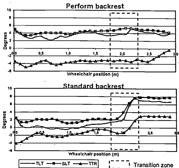
Figure 3. Evolution of parameters calculated for the two backrests with respect to the wheelchair position on the experimental pathway.
