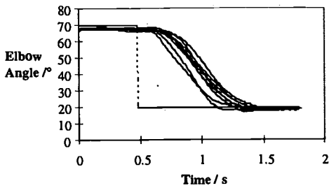
Figure 4: Actual (-) and target (--) elbow angle against time for ten physiotherapist assisted extension movements
