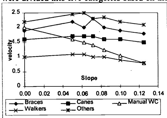
Figure 1. Velocity as a function of ramp slope.
