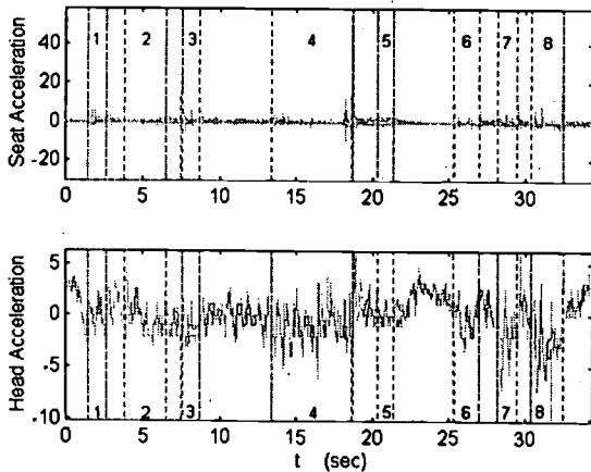
Figure 1. Acceleration signal during the course (trial 3 with cushion) passing 8 obstacles: 1, Dimple Strip; 2, carpet; 3, Door Threshold; 4, Ramp; 5, Rumble Strip; 6, Bump #1; 7, Bump #2; 8, Bump #3
