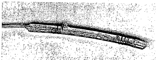
Figure 1. The IM electrode used in these studies consisted of a silicone tube. Two wires were passed through and wrapped around the tube to act as the anode and cathode.
