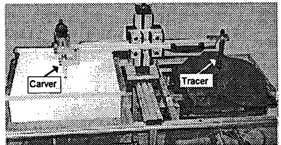
Figure1. The manual contour copier
