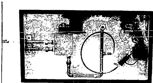
Fig. 1 Temperature control shower unit. The system includes: (1) motor; (2) mixing valve, (3) thermocouple, (4) PID controller, (5) transformer, (6) hot supply line, (7) cold supply line
