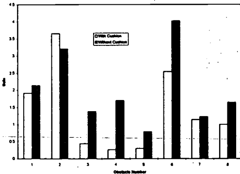
Figure 5. The energy transfer gain of the whole body acceleration (8 obstacles corresponding to the definitions in Figure 1)
