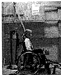
Figure 3: Laboratory Test Setup with Wheelchair Tiedown and Occupant Restraint System
