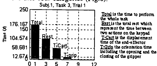
Fig.6 Analysis of the learning phase of Manus by quadruplegic patient
