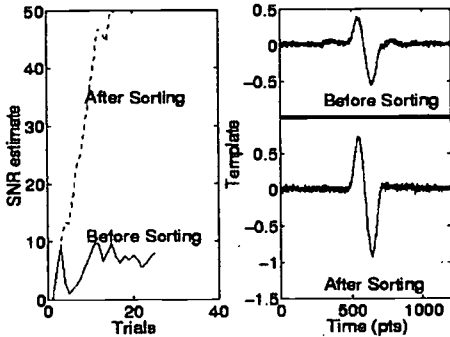
Figure 1 – Example of SNR estimate and template before and after sorting. A data set with temporal shifting was used. Note the "sidelobe" distortion of the template before sorting.
