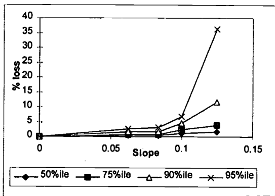
Figure 4. Distribution of loss as a function of ramp slope.
