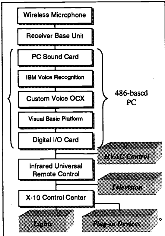
Figure #1 – Block Diagram of System
