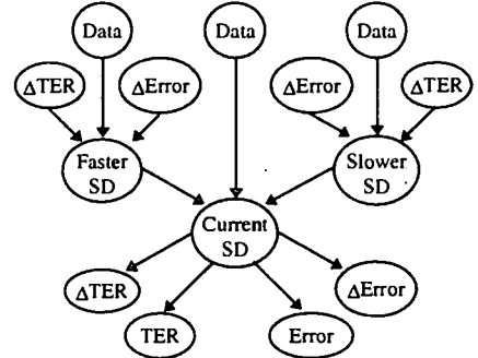
Figure 1. Bayesian network used to make adaptation decisions in row-column scanning system.
