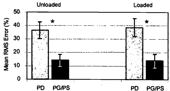
Figure 5: Mean RMS error +/- one standard deviation for all unloaded and loaded controller trials. Repeated-measures ANOVA showed that the PG/PS controller had a significantly (*, p-value < 0.05) lower RMS error than the PD controller.
