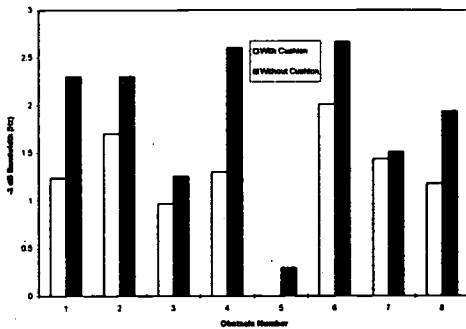
Figure 4. -3 dB band width of the whole body acceleration transfer system (8 obstacles corresponding to the definitions in Figure 1)
