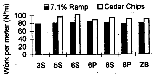
Figure 1. Work required on the ramp and cedar chips
