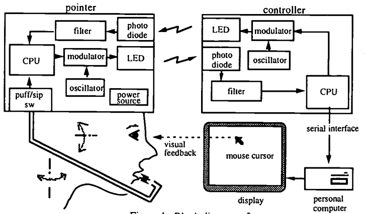
Figure 1. Block diagram of system
