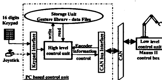
Figure 1: Hardware organization
