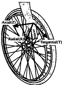
Fig.1 - Coordinate System
