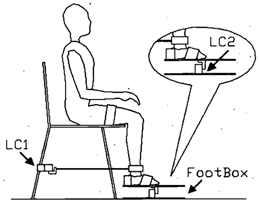
Fig. 1 IVES Setup
