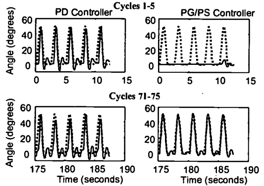
Figure 3: Example trials of the best PD Controller and the best PG/PS controller for the first 5 cycles and the last 5 cycles. Note as the trial continues, the PG/PS controller improves performance, but the PD controller (thin line) only maintains performance
