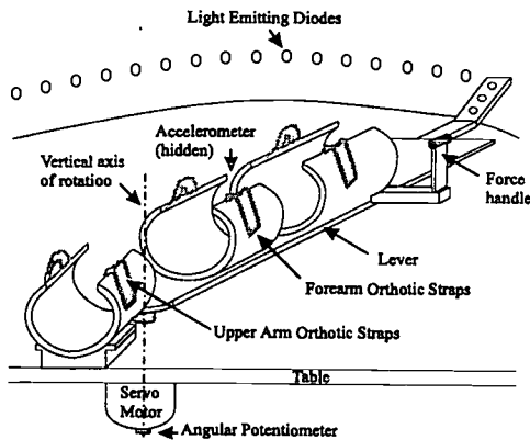
Figure 1: Experimental apparatus
