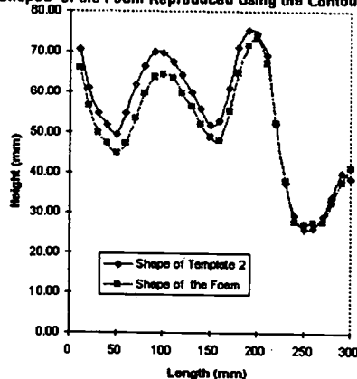
Comparison Between the Shape of Template 3 and the Shaped of the Foam Reproduced Using the Contour Copier
