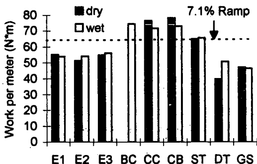
Figure 2. Work required for turning propulsion
