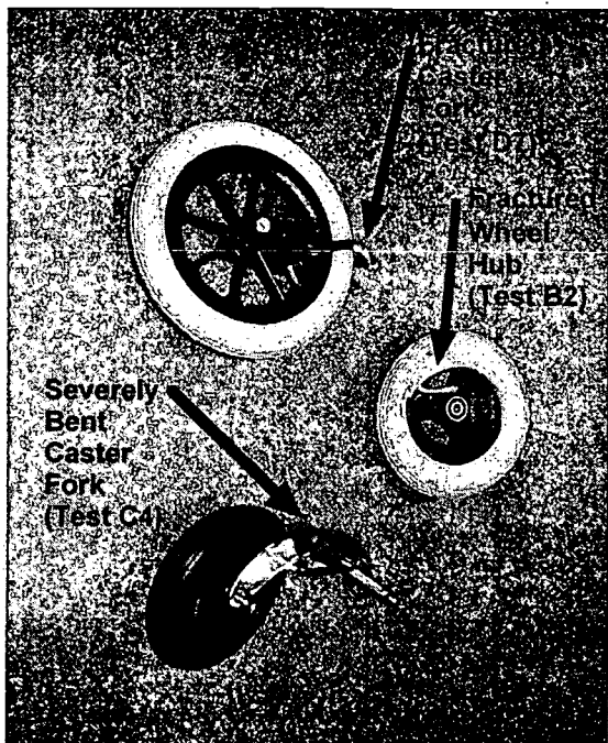
Figure 3 Select Caster Assembly Failures
