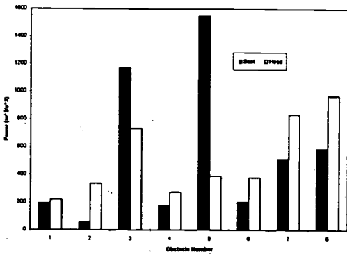
Figure 3. The power of head and seat acceleration for different obstacles ( 8 obstacles corresponding to the definitions in Figure 1 )
