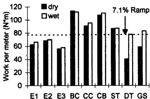
Figure 1. Work required for straight propulsion
