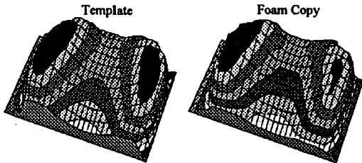
Figure 3b. 3-D mesh representations of the headrest
