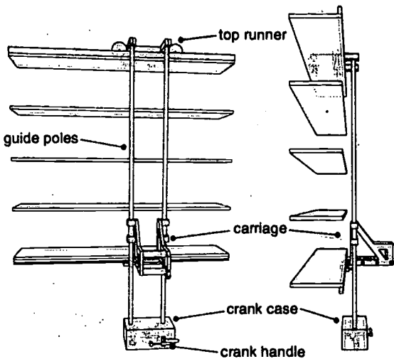
Figure 1 The final design.
