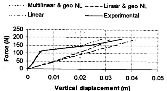
Figure 2: Validation results with Neocor HR35; geo NL: geometric nonlinearities
